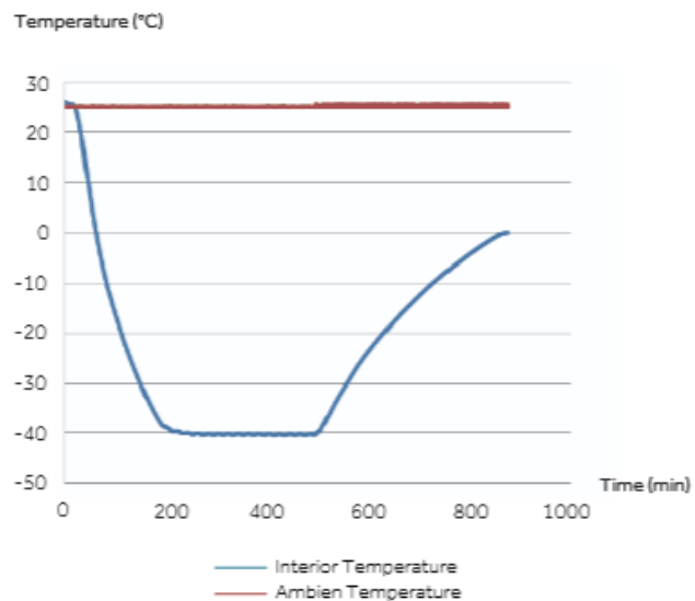
DW-40L528D Typical Performance Characteristics at 25°C Ambient
