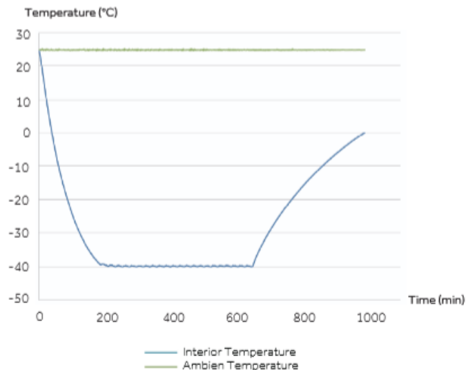
DW-40L418D Typical Performance Characteristics at 25°C Ambient
