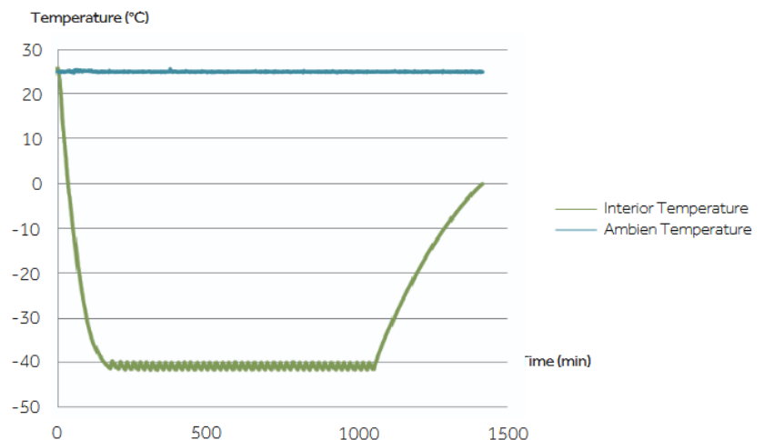
DW-40L298J Typical Performance Characteristics at 25°C Ambient
