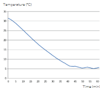
HYC-410 Cooling down (ambient 32°C)
