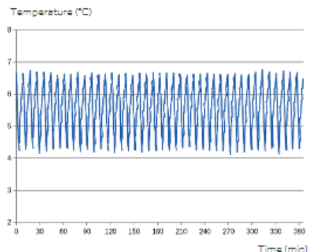
HYC-410 Stability (ambient 25°C)
