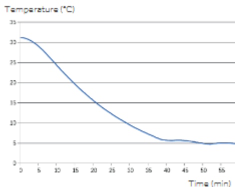
HYC-118A Cooling down (ambient 32°C)
