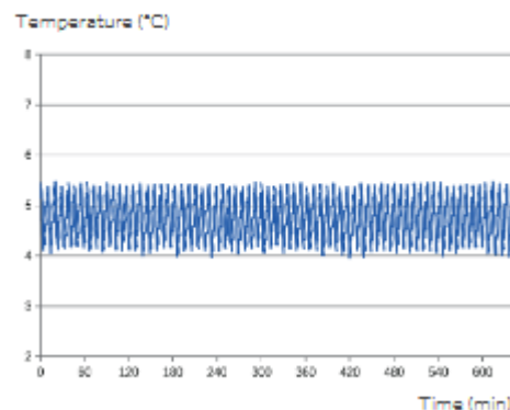
HYC-118A Stability (ambient 25°C)
